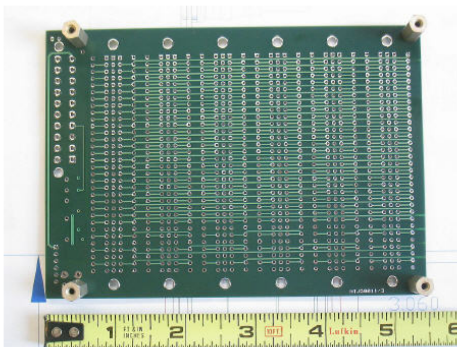
Bare board bottom side (photo Phil Covington, N8VB; scale shows Inches )
